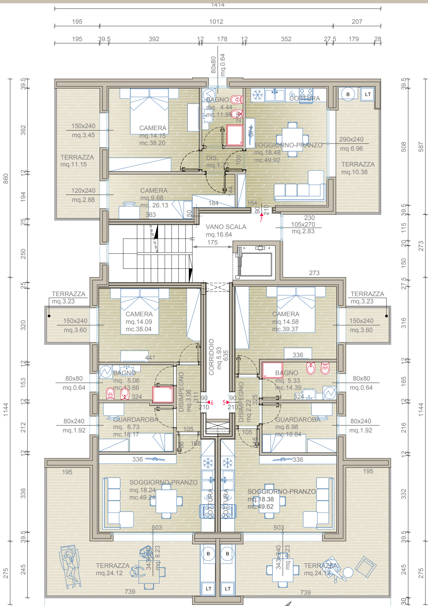
PIANTA PIANO II°
